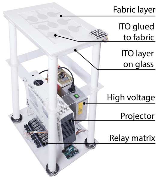
Figure 2. TableHop consists of a top layer of fabric with an ITO array, an ITO and glass bottom layer, high-voltage supply, relay matrix, microcontroller, a rear projector, and a user tracking device for interaction.
